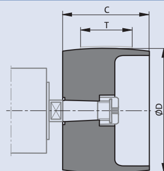
Pulley for interface V
