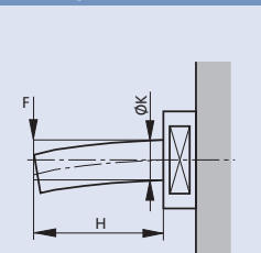
Quill stiffness
